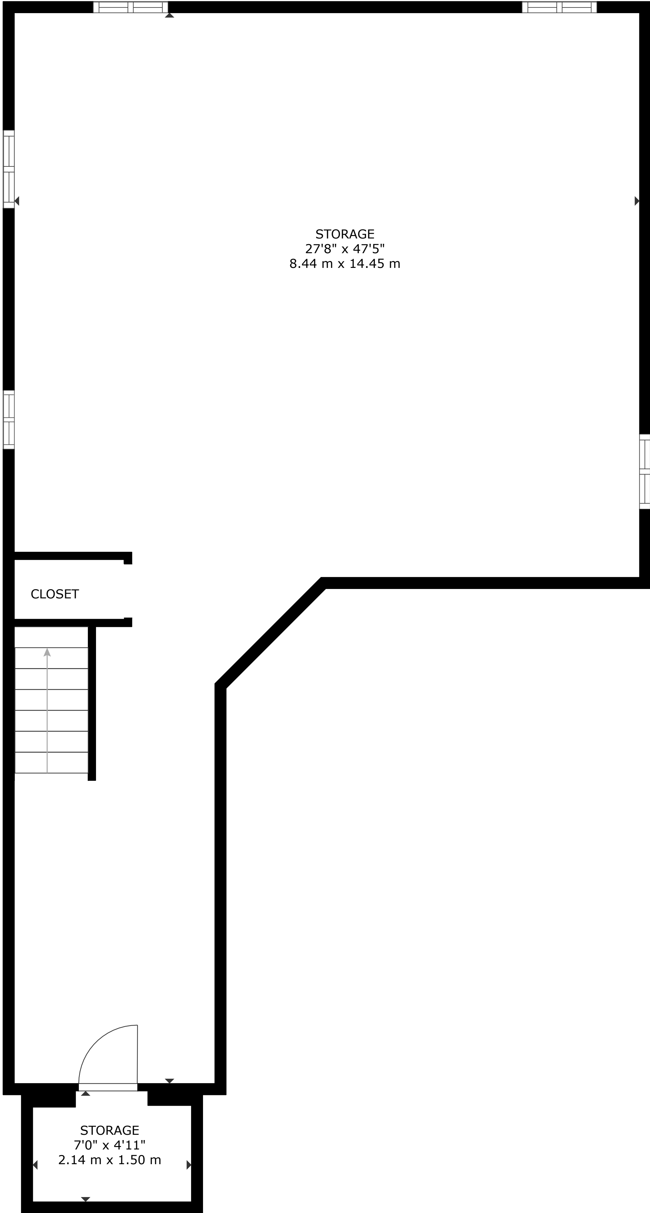
FLOOR 1
